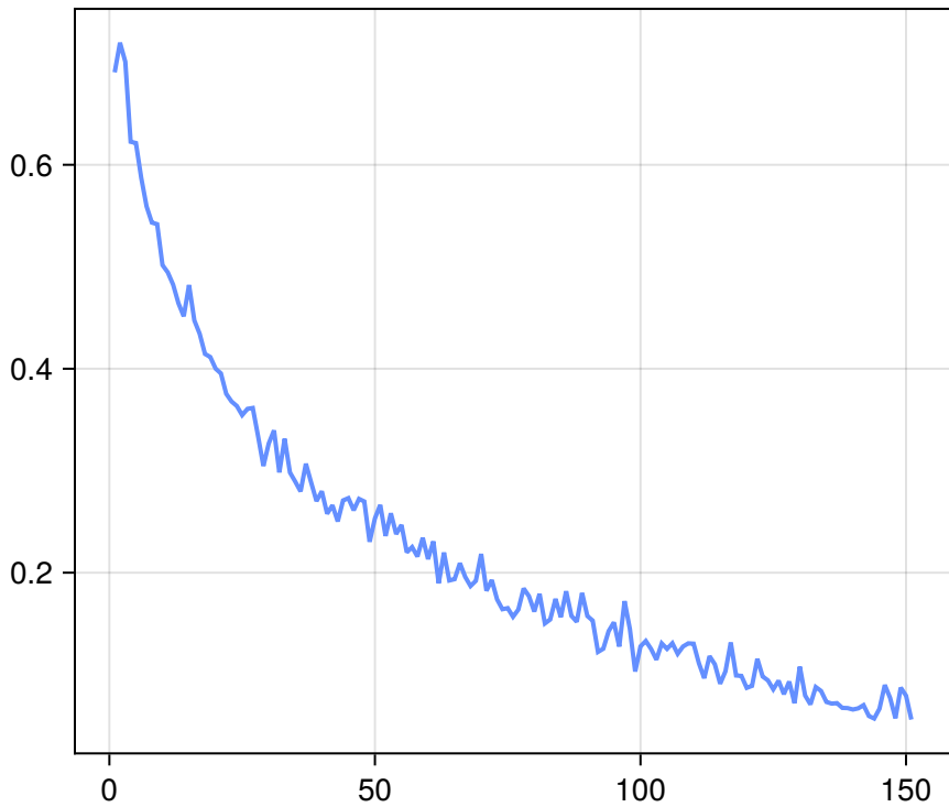
Outer Fold 5
