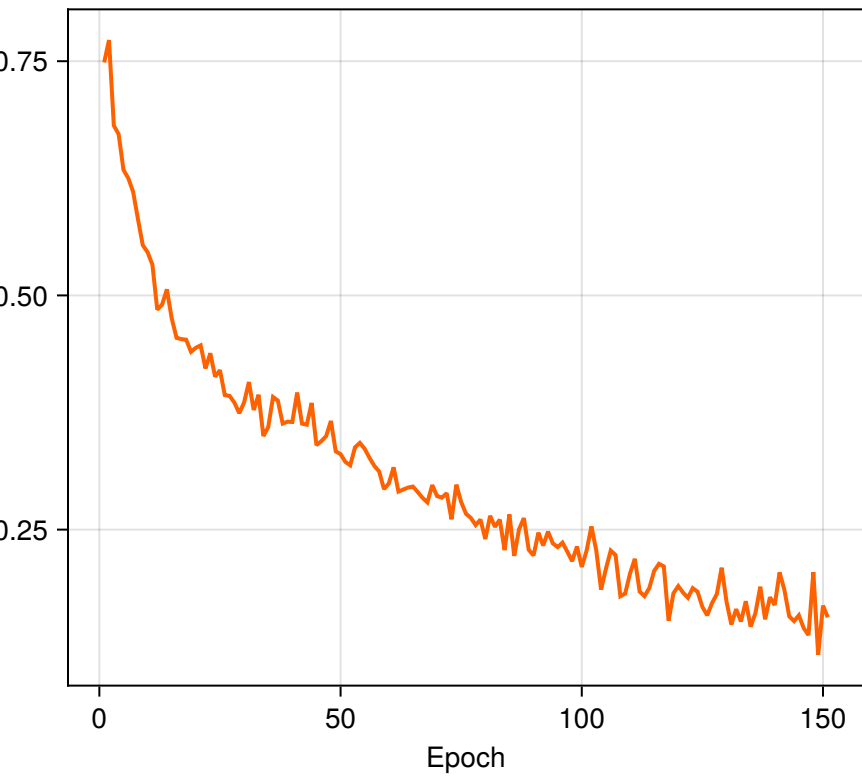
Outer Fold 5
