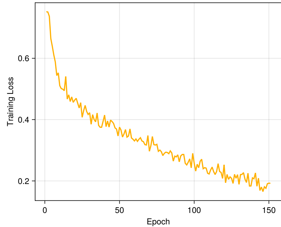
Outer Fold 4
